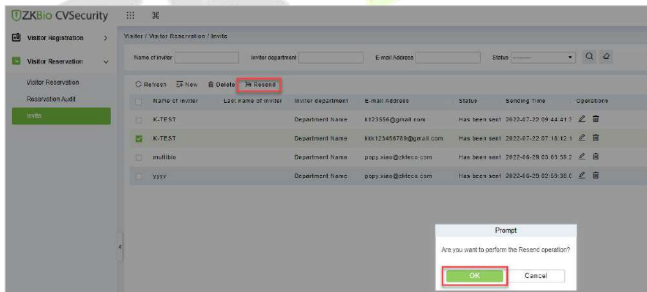
Figure 8- 25 Resend Invitations
