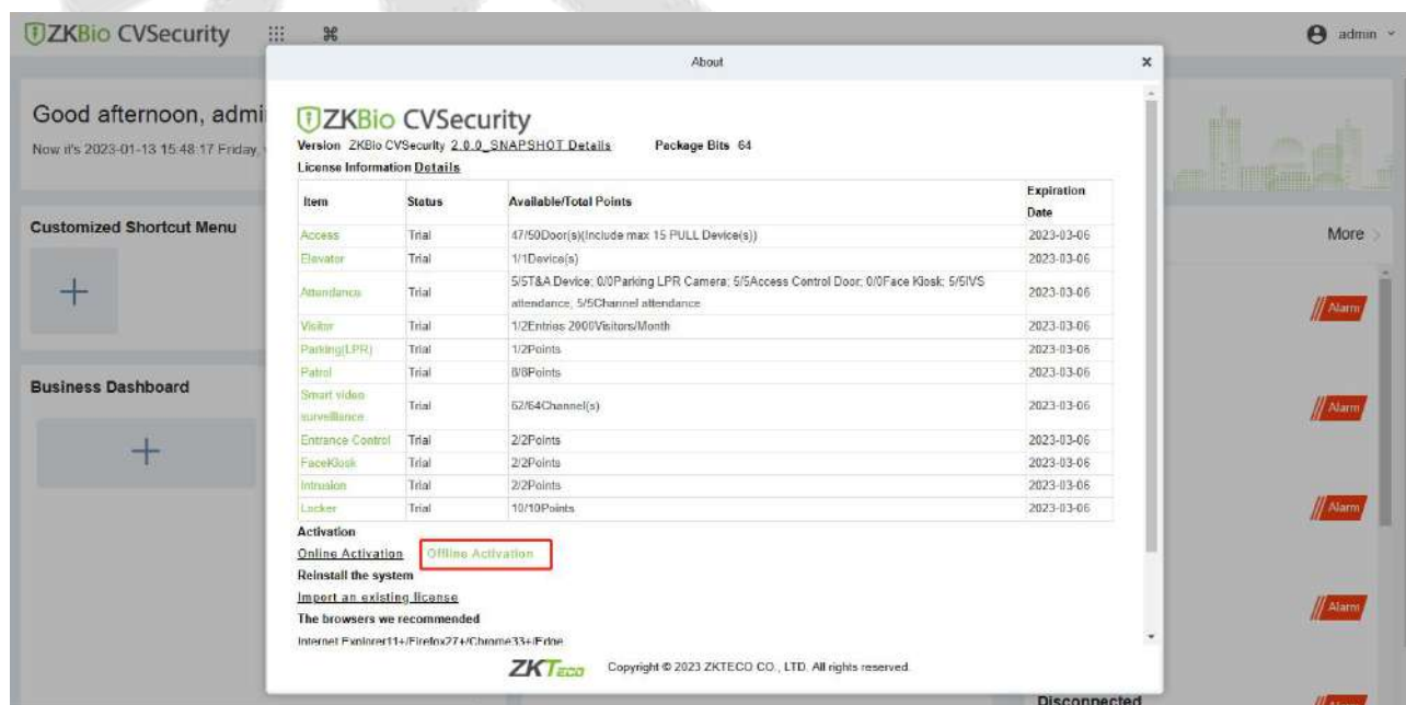
Figure 1- 34 Offline Activation
