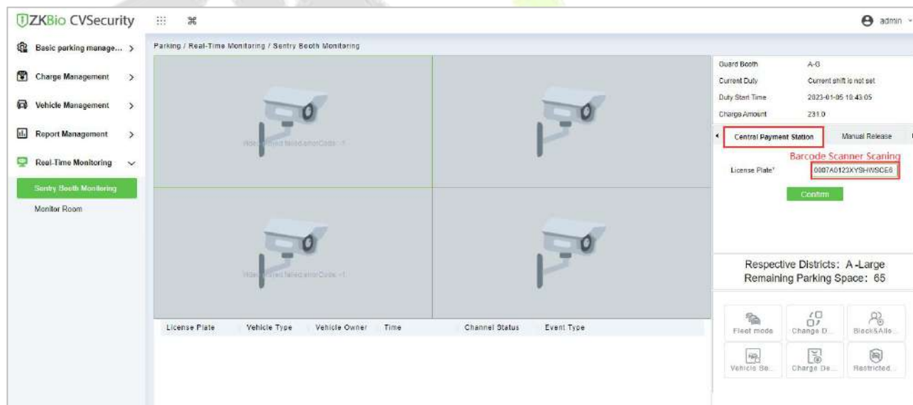
Figure 7- 73 Overstay Rule
