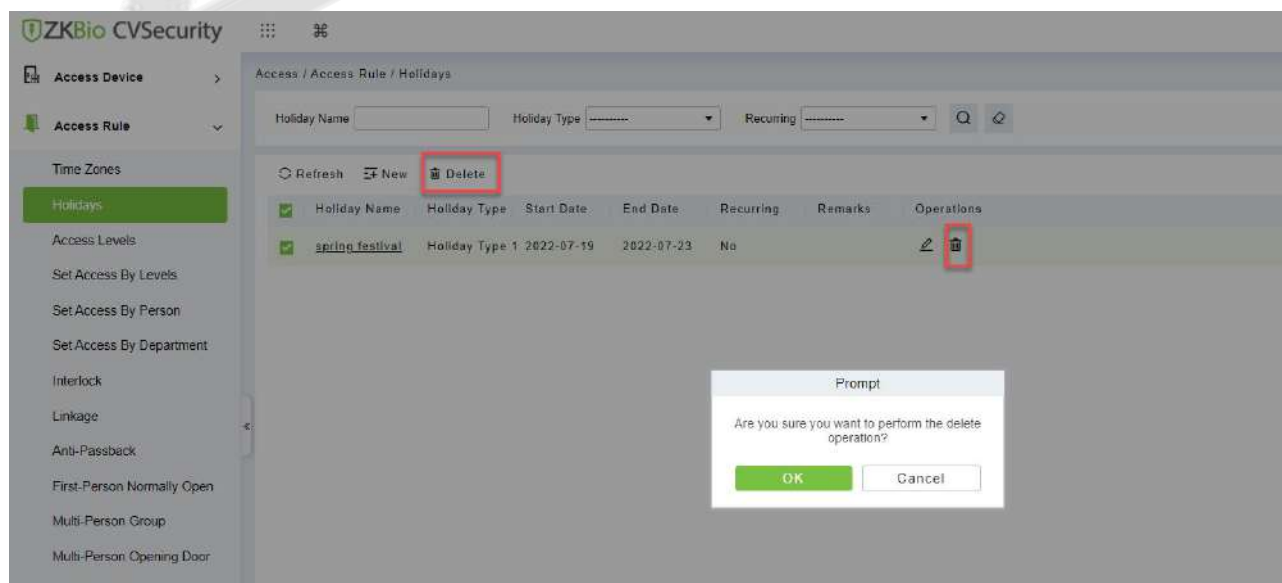
Figure 3- 46 Holiday Delete
