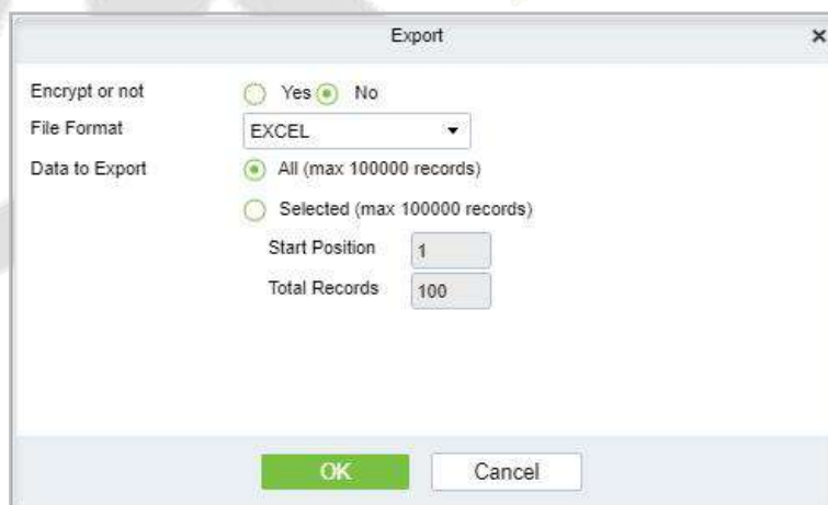
Figure 8- 14 Export Interface
