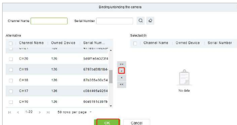
Figure 16- 6 Binding Camera
