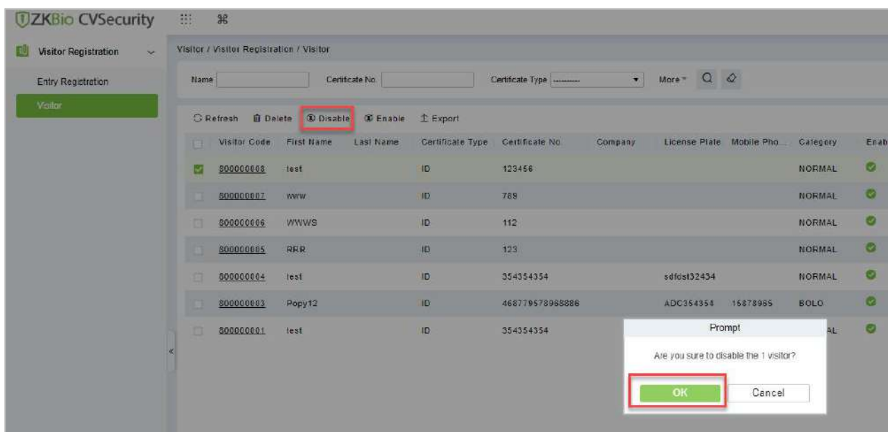
Figure 8- 11 Disabling Visitor
