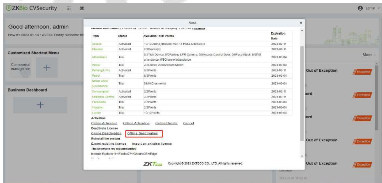
Figure 1- 14 Offline Deactivation
