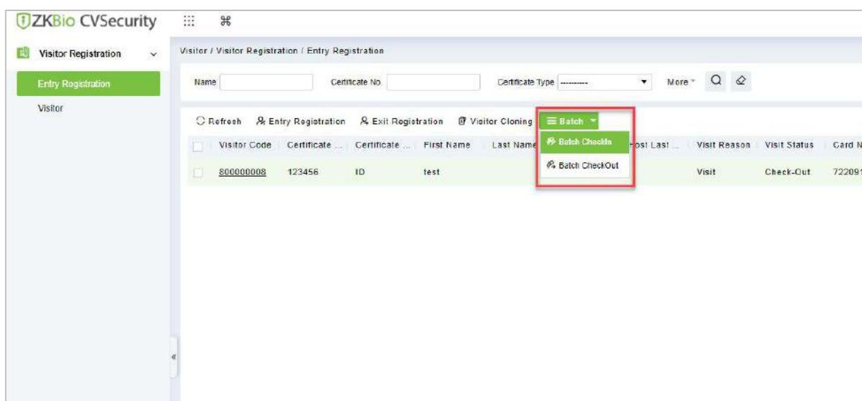
Figure 8- 6 Batch Interface
