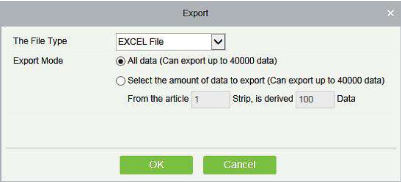
Figure 3- 108 Export
