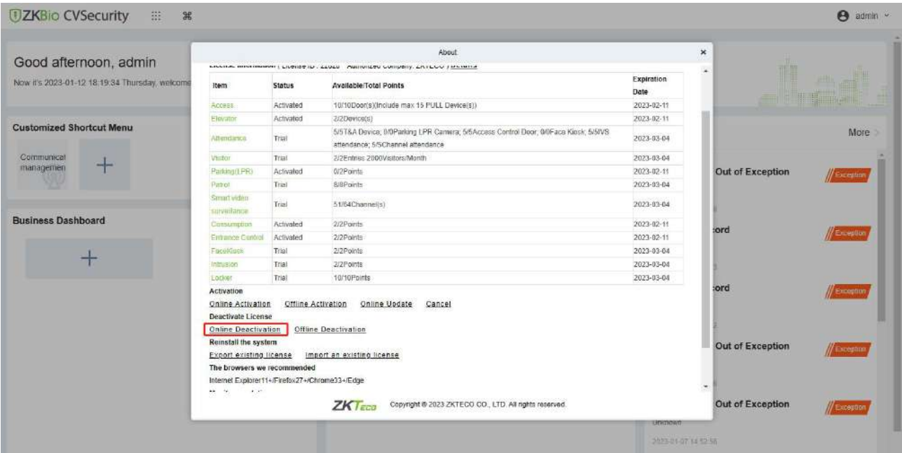
Figure 1- 21 Online Deactivation
