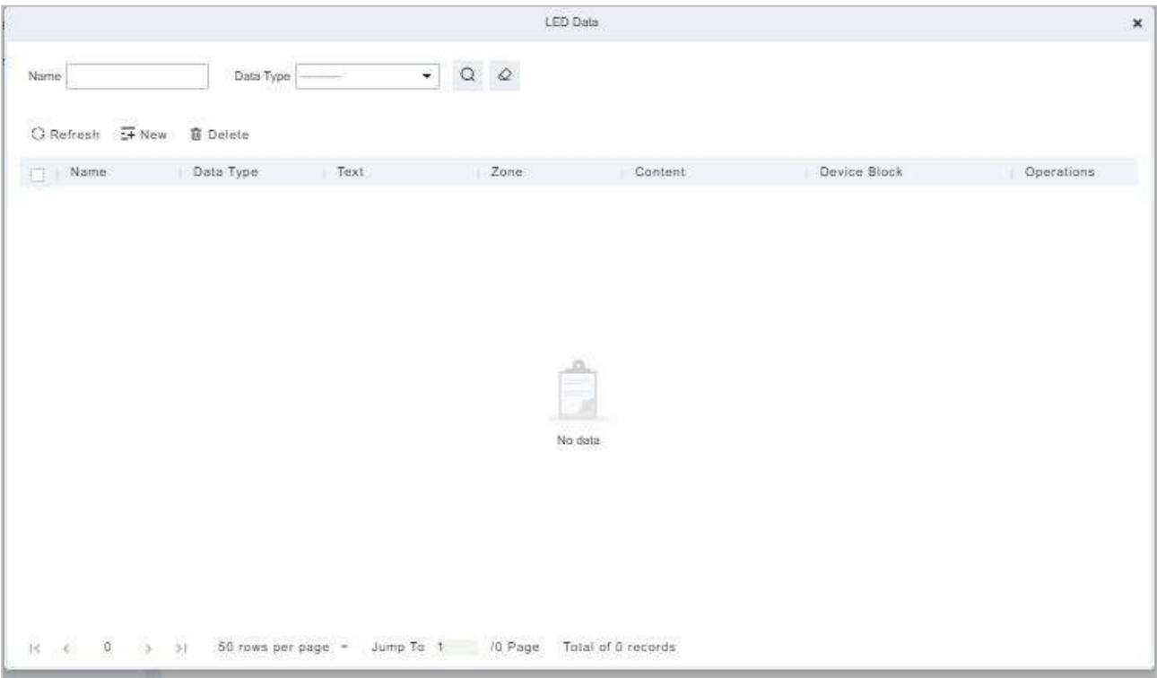
Figure 18- 63 LED Data
