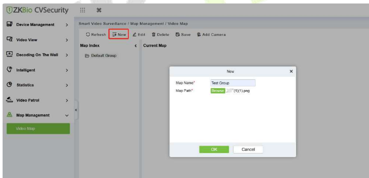
Figure 5- 67 Video Map
