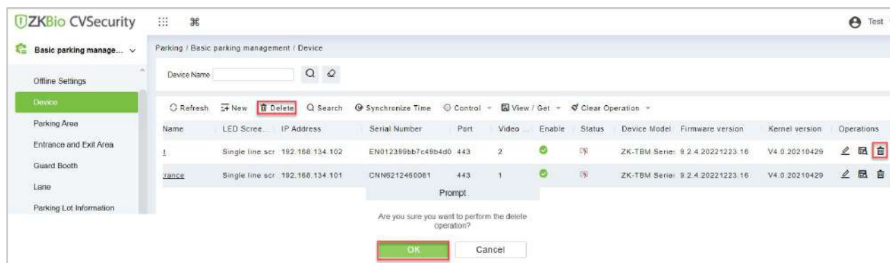
Figure 7- 59 Delete device
