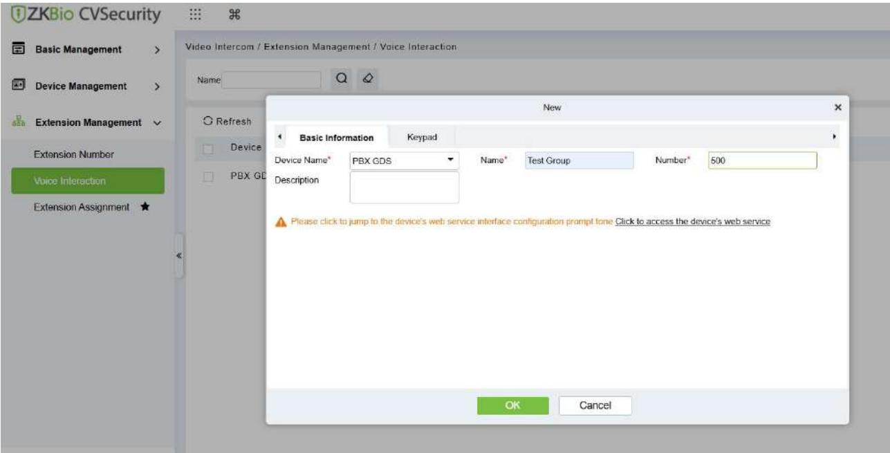
Figure 4- 40 Voice Interaction
