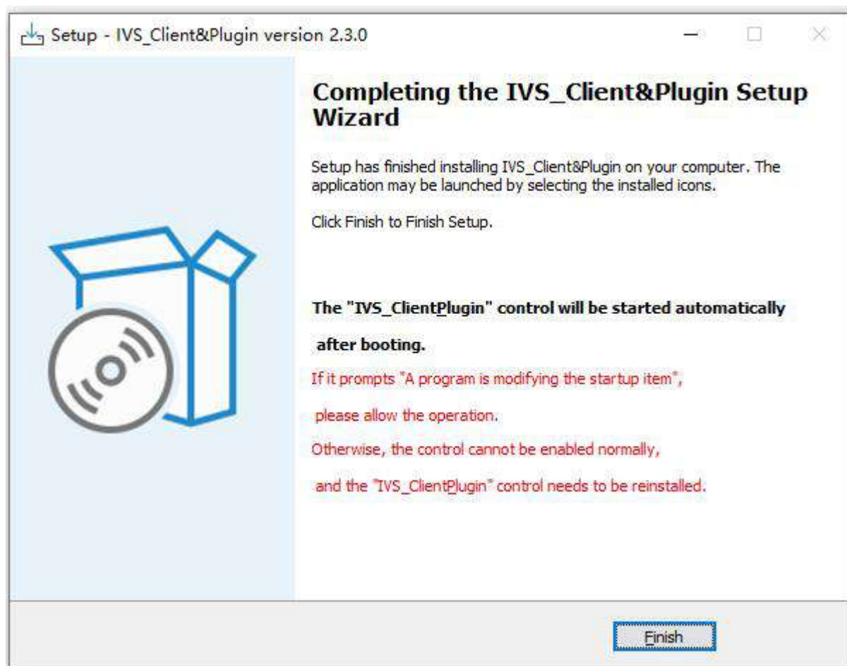
Figure 5- 83 Finish Installation
