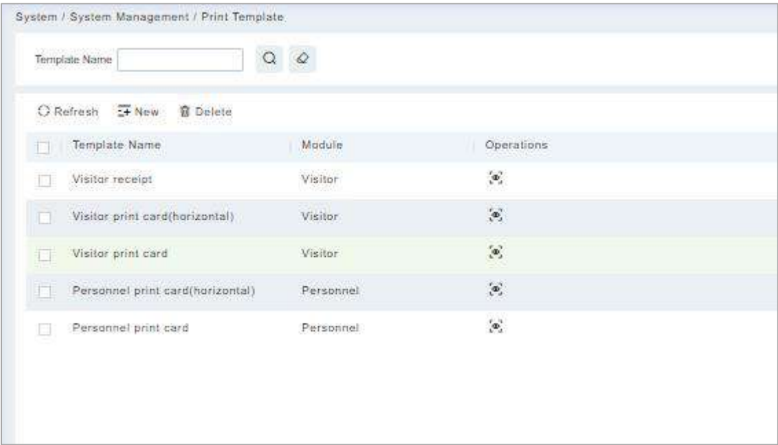
Figure 18- 22 Print Template
