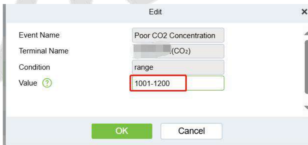
Figure 17- 13 Event Type
