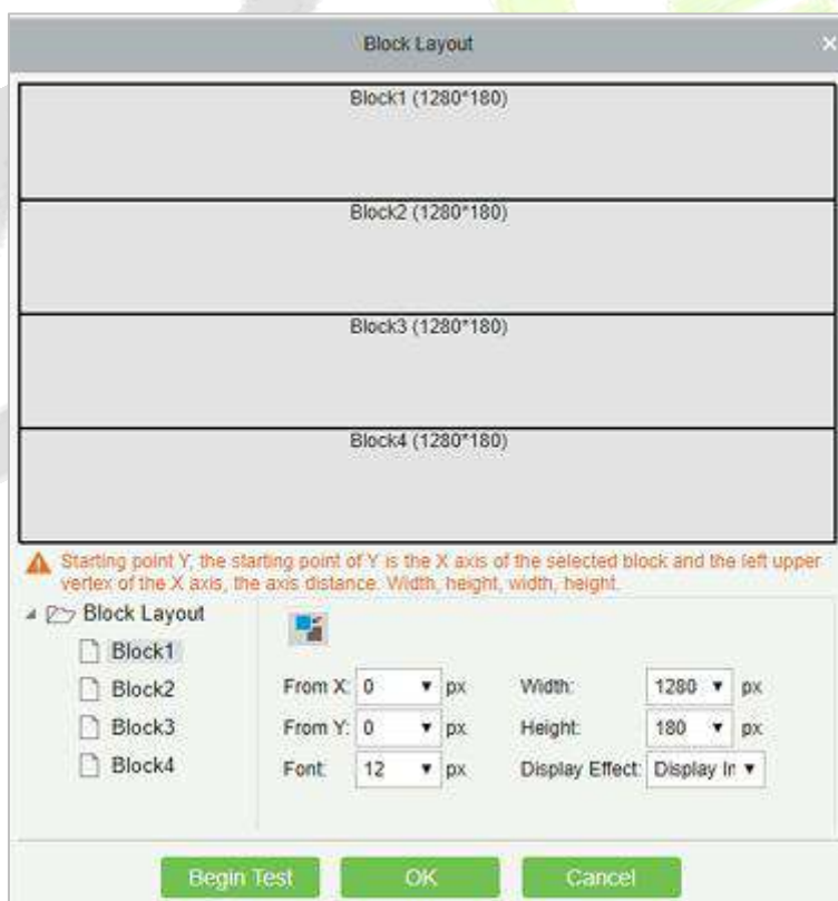
Figure 18- 62 Block Layout
