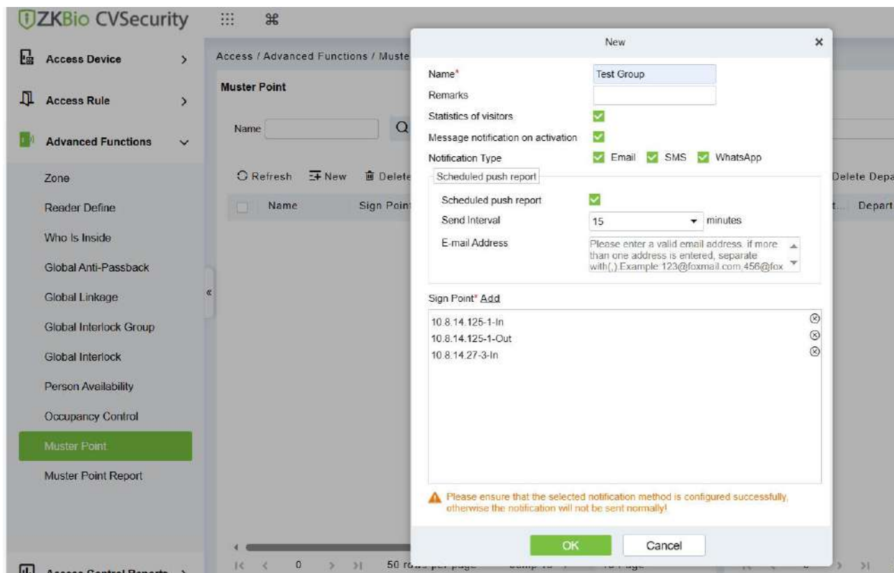
Figure 3- 128 Sign Point
