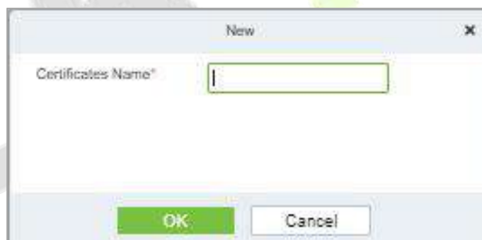
Figure 18- 21 New Option
