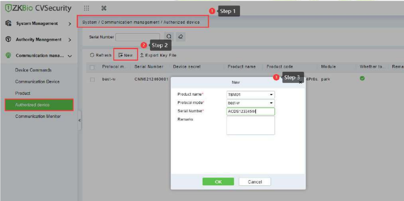
Figure 7- 43 Authorized Device
