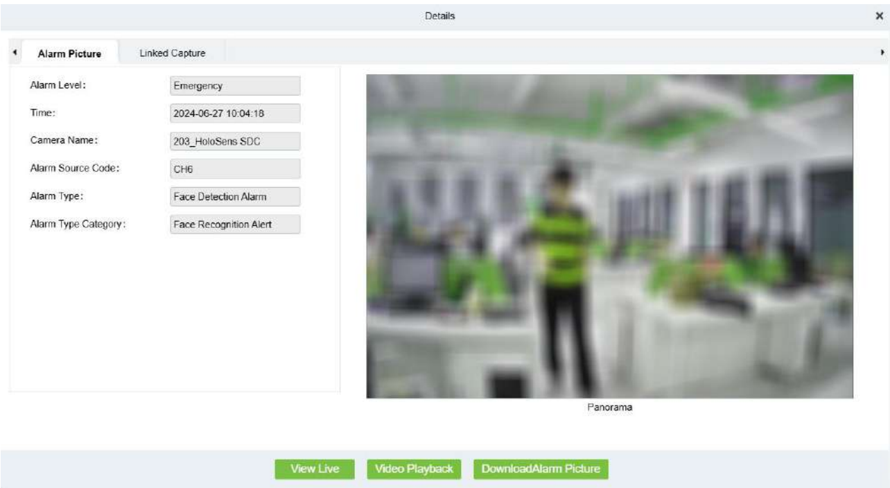
Figure 5- 39 Alarm Detail
