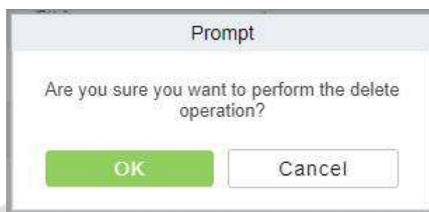
Figure 5- 59 Prompt
