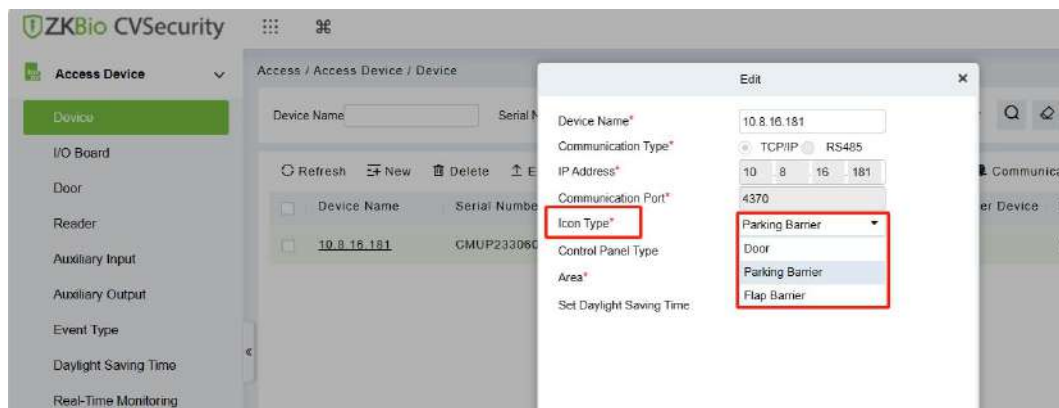
Figure 3- 34 Icon Type
