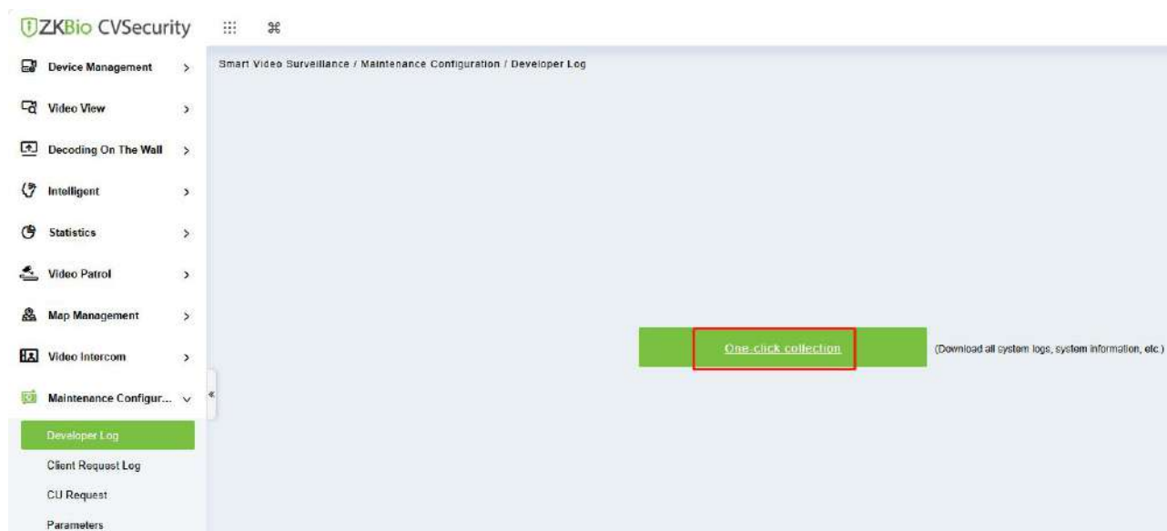
Figure 5- 73 One-Click Collection
