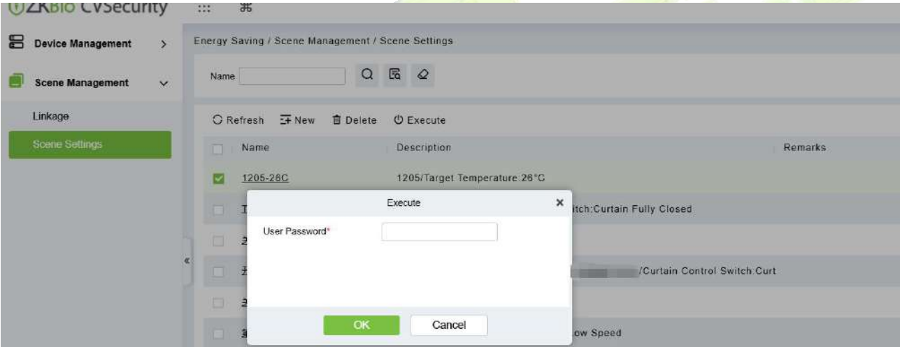
Figure 17- 20 Execute Scene
