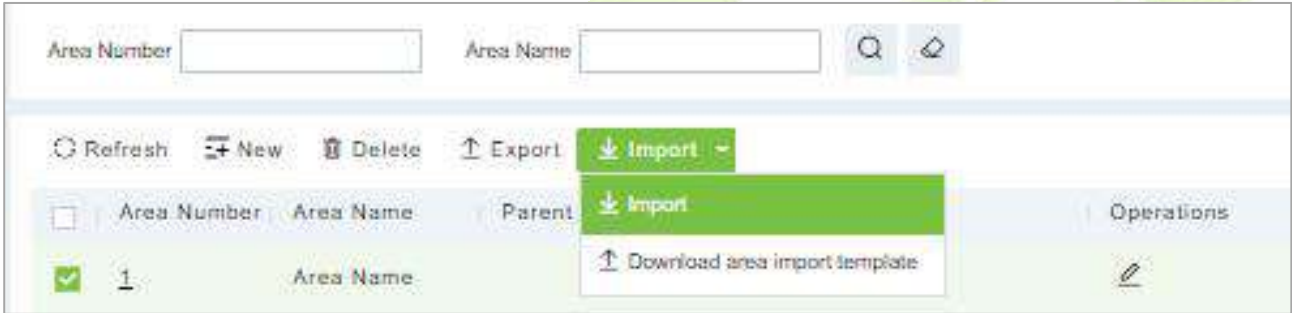
Figure 18- 9 Import Interface
