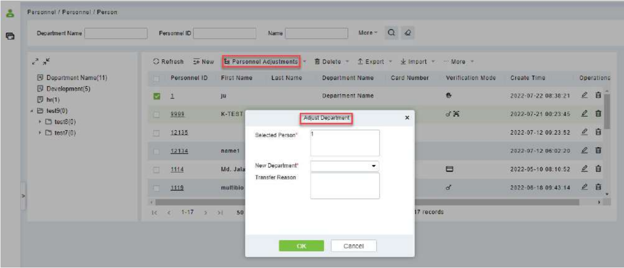
Figure 2- 17 Adjust Department
