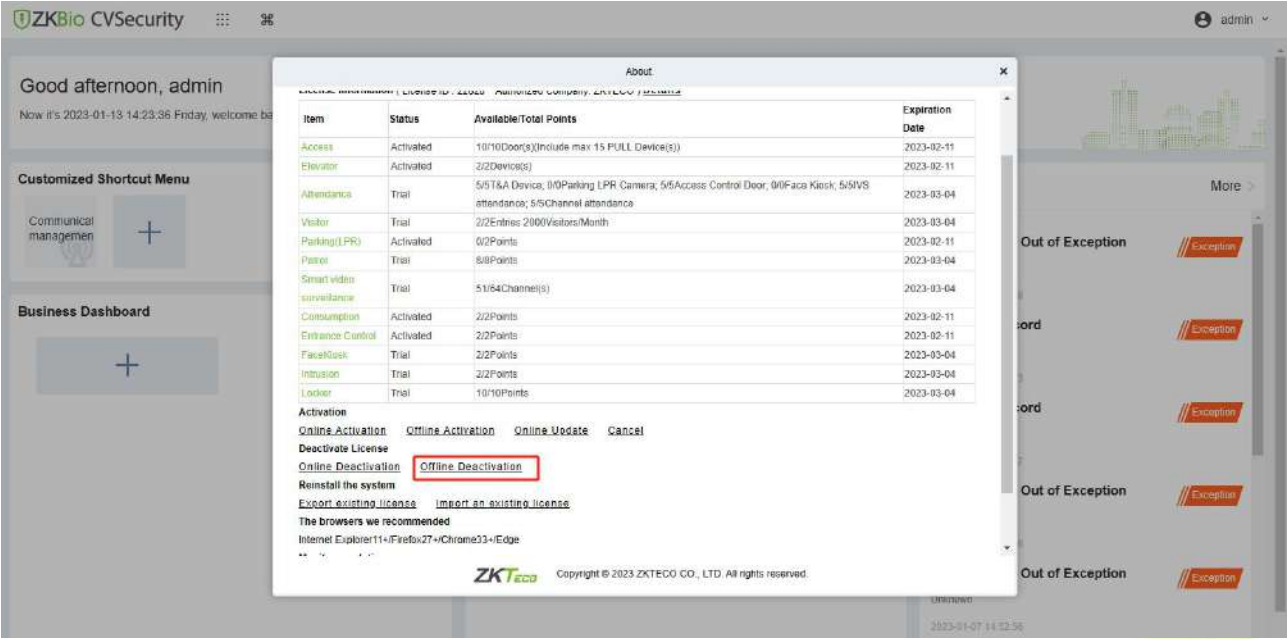
Figure 1- 29 Offline Deactivation
