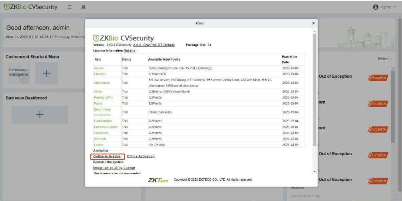
Figure 1- 11 Online Activation
