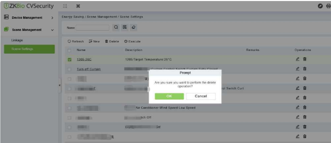
Figure 17- 19 Delete Scene
