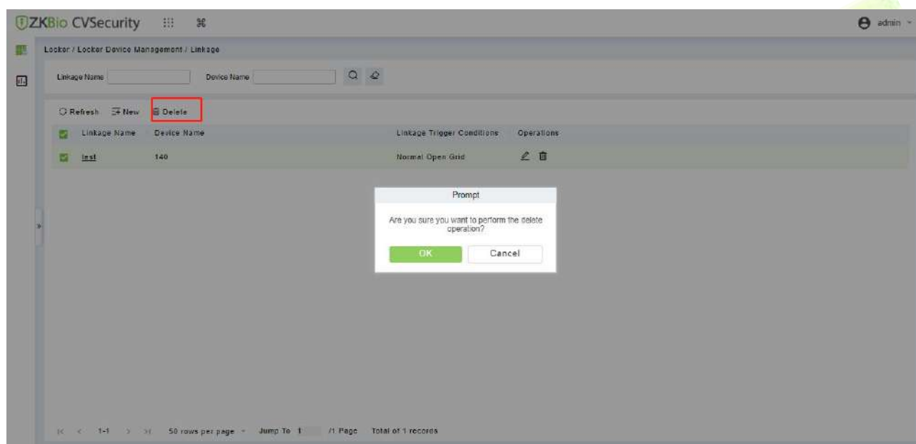
Figure 16- 17 Delete Linkage
