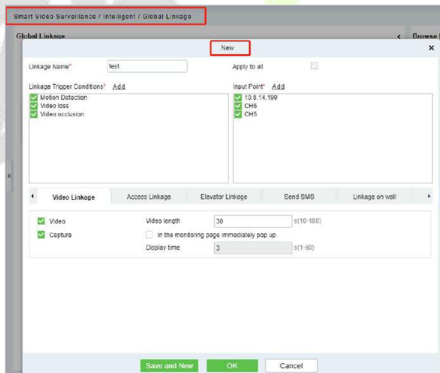
Figure 5- 42 Global Linkage
