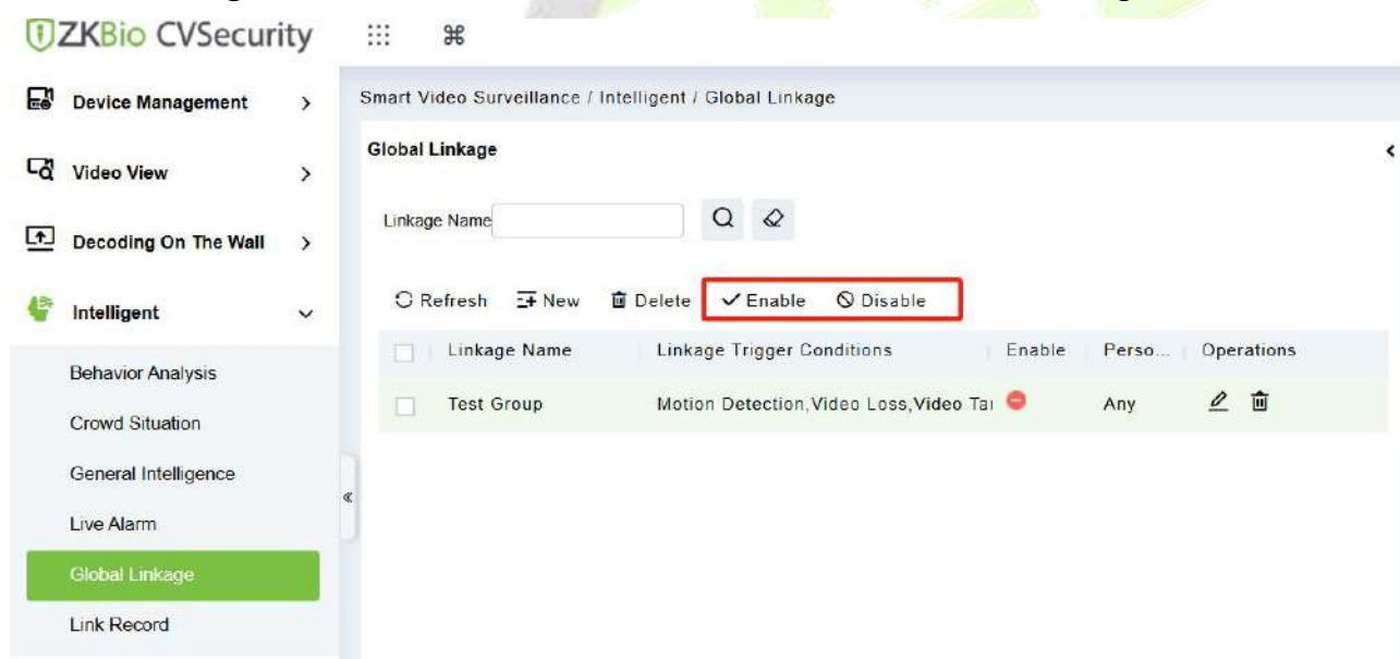
Figure 5- 43 Enable/disable Linkage
