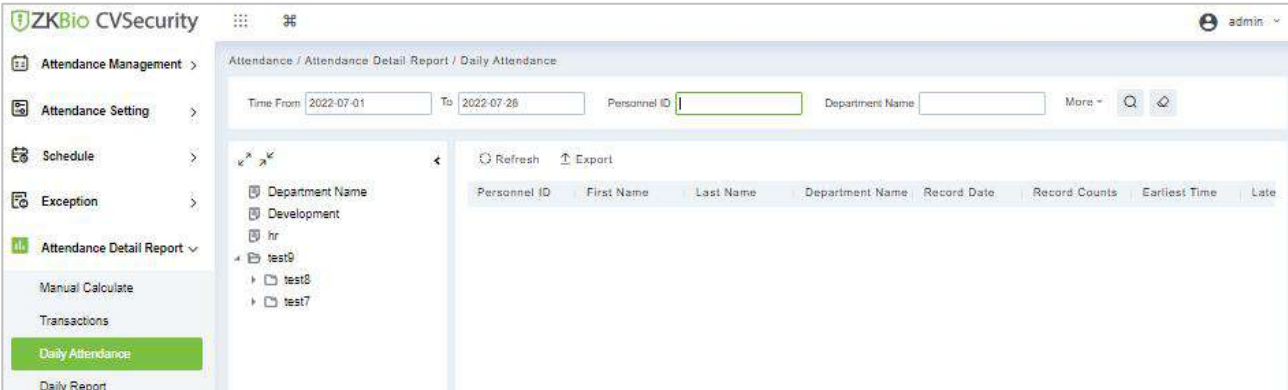
Figure 6- 48 Daily Attendance
