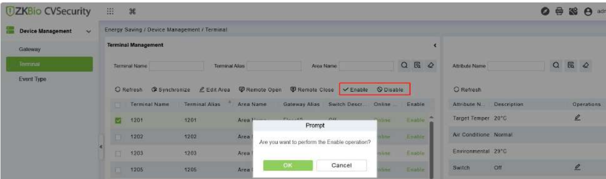
Figure 17- 9 Enable / Disable
