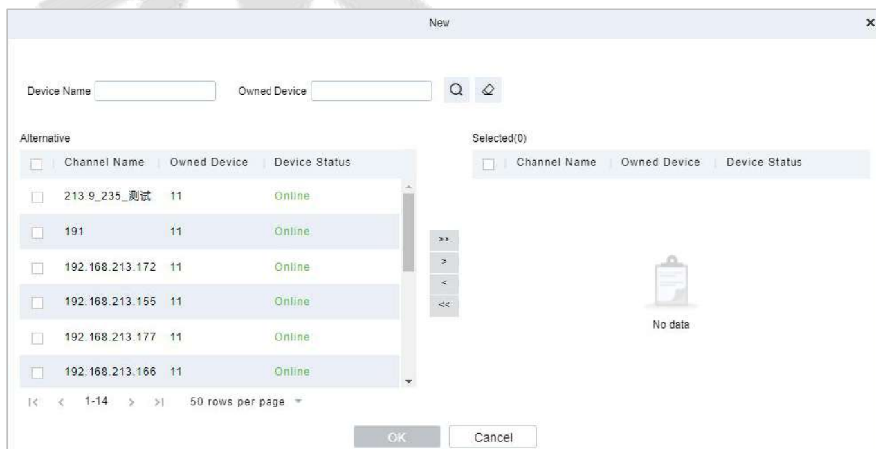
Figure 5- 12 Camera Grouping
