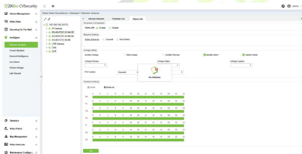
Figure 5- 23 Non-Smart Cameras
