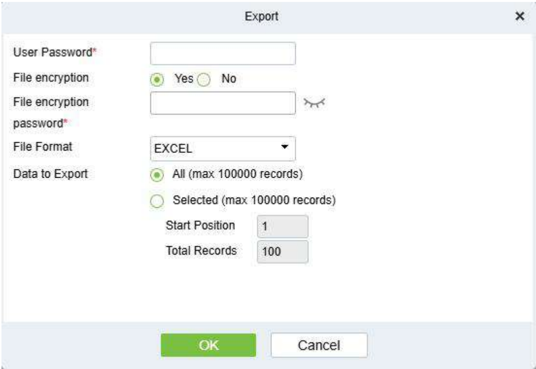
Figure 5- 77 Export
