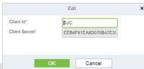
Figure 18- 36 Edit Option
