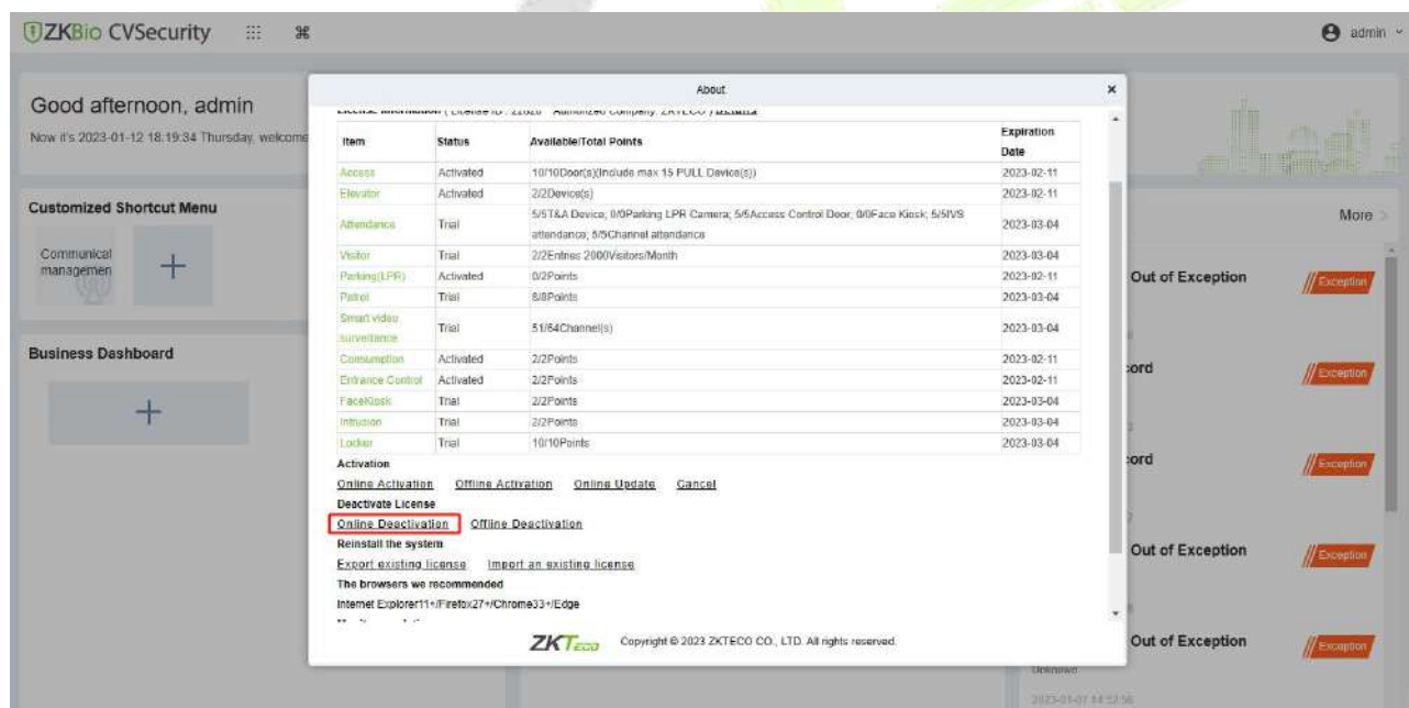
Figure 1- 8 Online Deactivation
