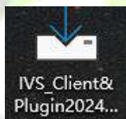
Figure 5- 79 Install Package
