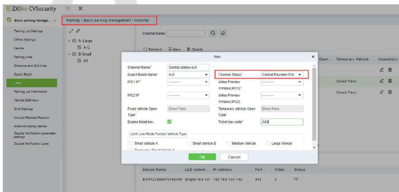
Figure 7- 71 9-65 Channel Setting (2)
