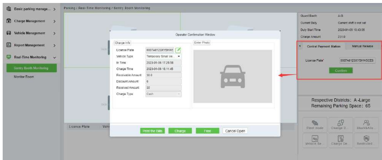
Figure 7- 74 Overstay Rule (2)
