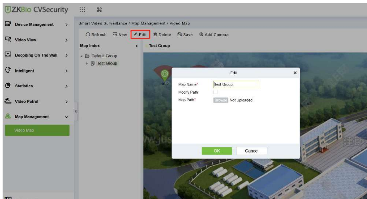
Figure 5- 71 Edit Map
